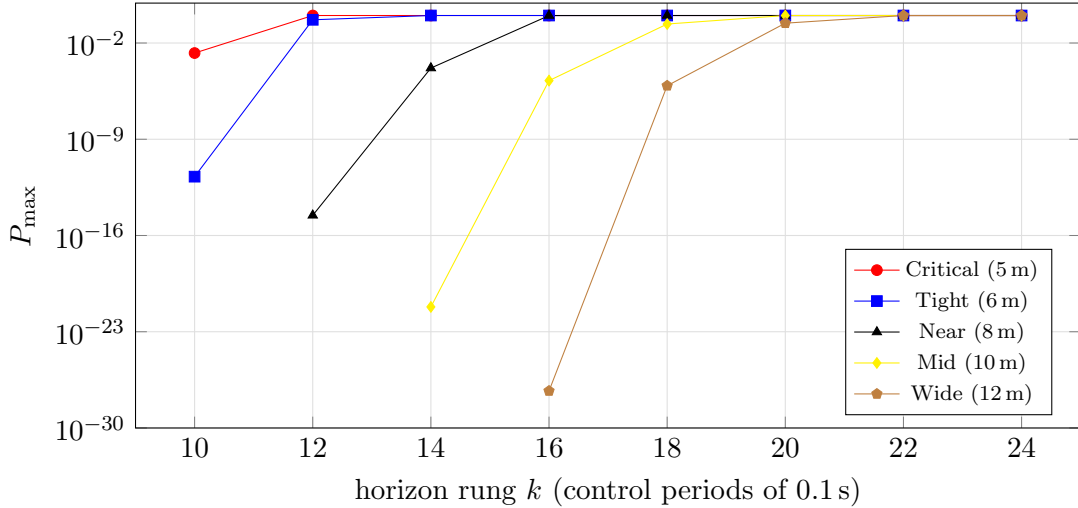
Figure 19: Worst-case crash probability against the horizon rung for the Following family, logarithmic vertical axis. Each point is one checker result on the certified extra_fine encoding; rungs at which P_{\max} is exactly 0 cannot be drawn on a logarithmic axis and are omitted (Table 6 records them). The curves shift right with the starting gap without crossing.
