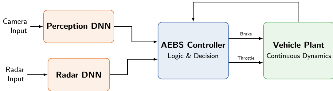
Figure 18: Case-study system architecture. Under perfect perception only the plant is abstracted.
