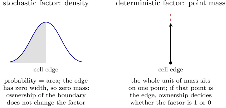
Figure 14: The two factor types of the product kernel. A density factor (left) assigns zero probability to any single point, so which cell owns a shared boundary does not affect its value. A point-mass factor (right) concentrates the whole unit of mass on one point; when the image lands exactly on a shared boundary, the half-open convention of Section 4.1 determines which cell receives the mass, which is why the upper inequality in (17) must be strict.
