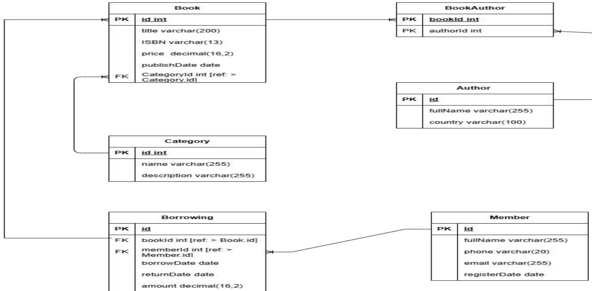
ERD Library System
