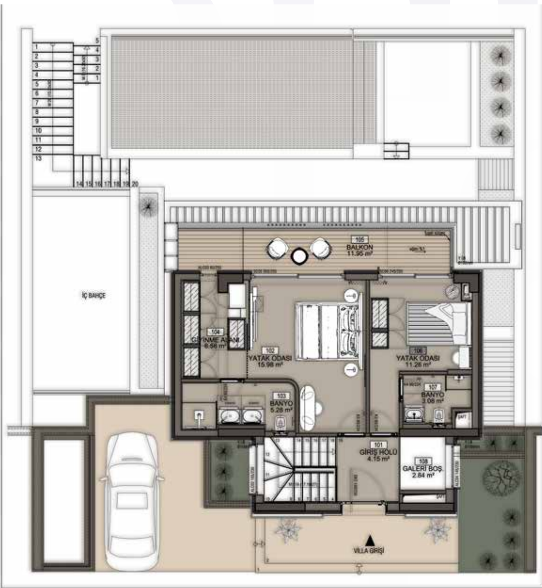
A Block First Floor Plan
