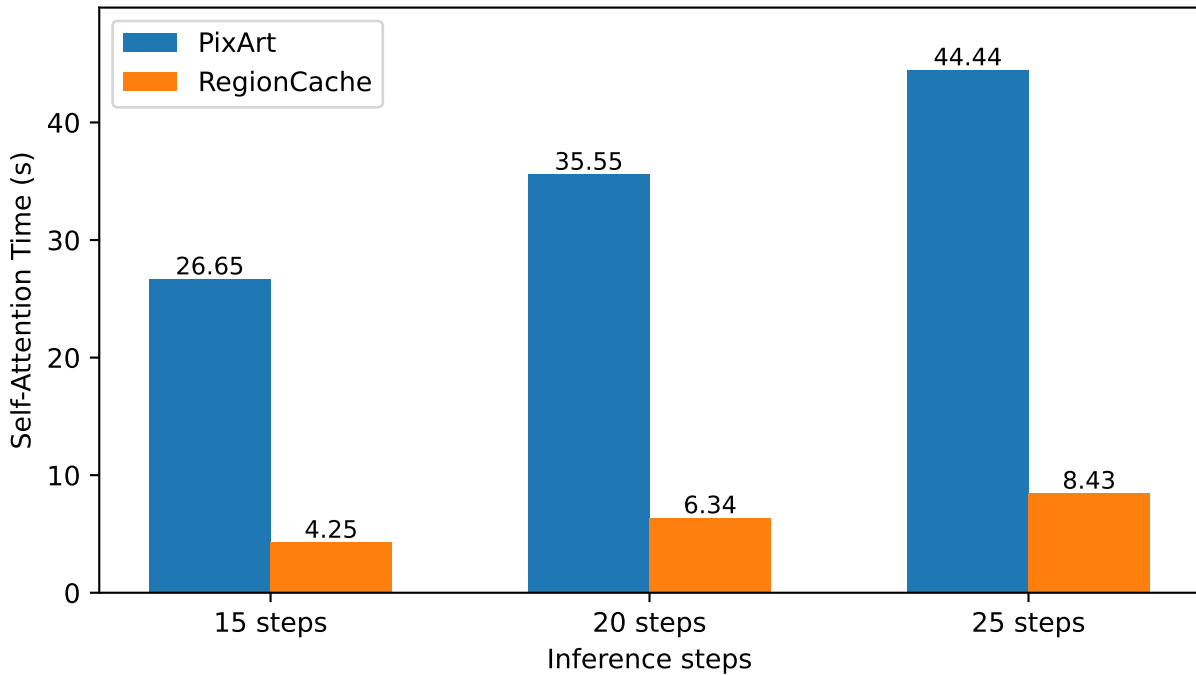
Self-Attention Time Comparison (2048x2048)
