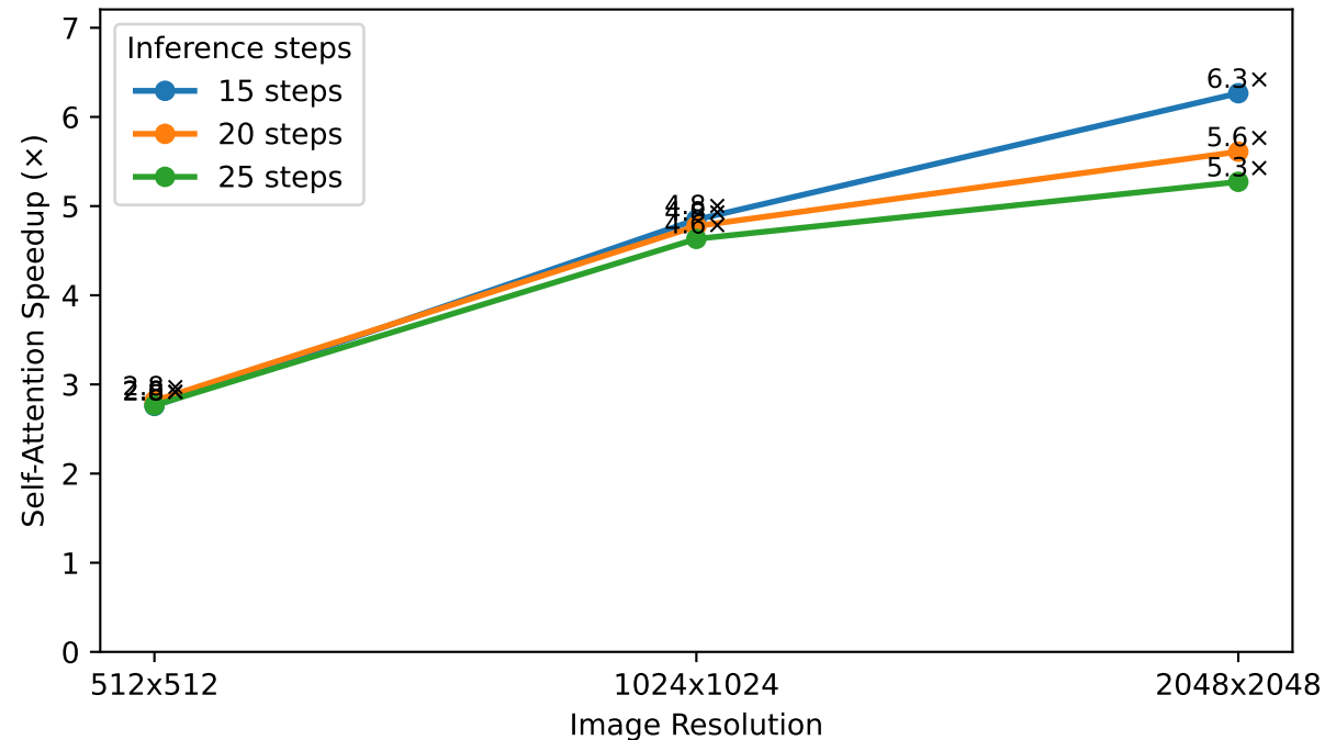
Speedup vs Image Resolution
