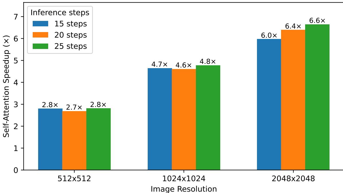
Self-Attention Speedup across Image Resolutions
