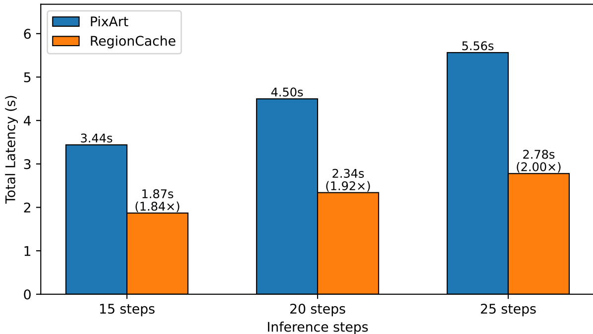
End-to-End Latency Comparison (1024x1024)
