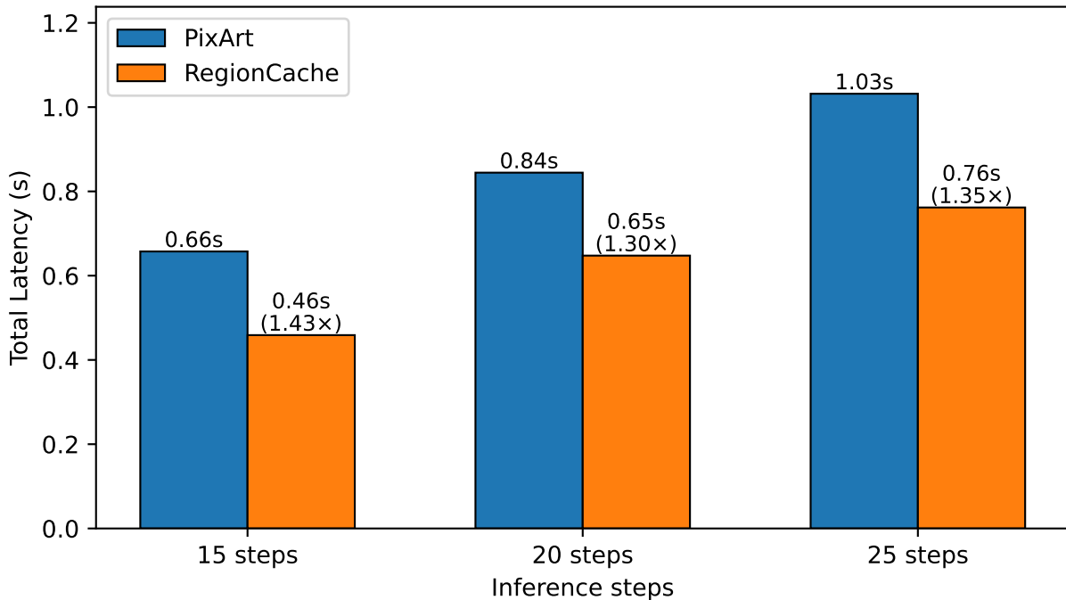
End-to-End Latency Comparison (512x512)
