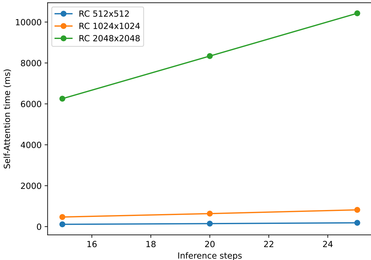
RegionCache: Self-Attention time vs steps
