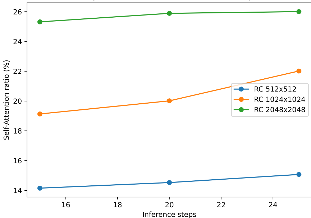
RegionCache: Self-Attention ratio vs steps
