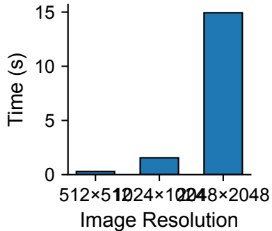
Full Attention Time
