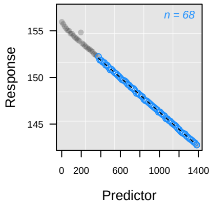
-- L_{pc} Rank 1: y = 155.53 - 0.0093 \cdot x
