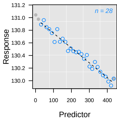
-- L pc Rank 1: y = 130.99 - 0.0024 \cdot x
