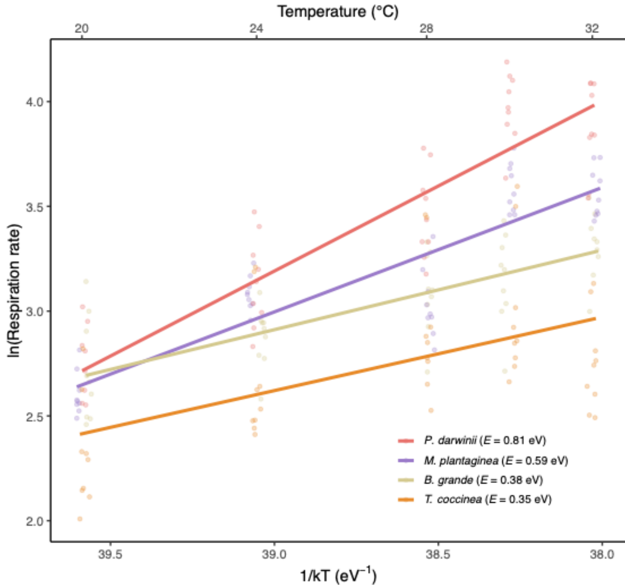
Fig. 3. Arrhenius regressions of dark respiration rate against inverse absolute temperature ( 1/kT ) for four Galápagos cnidarian species across the shared rising portion of the thermal response (20–32°C). Points show individual replicate measurements; lines are species mean regression slopes. Steeper slopes indicate higher activation energy ( E ) and greater thermal sensitivity. The top axis shows corresponding temperatures in °C.
