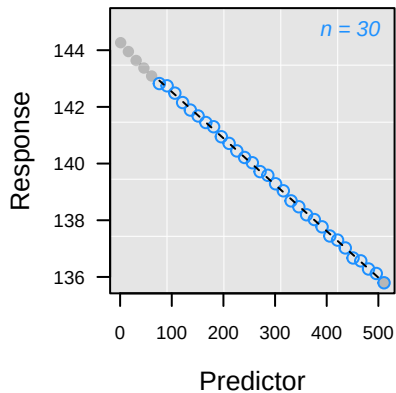
-- L pc Rank 1: y = 144.17 - 0.0164 \cdot x
