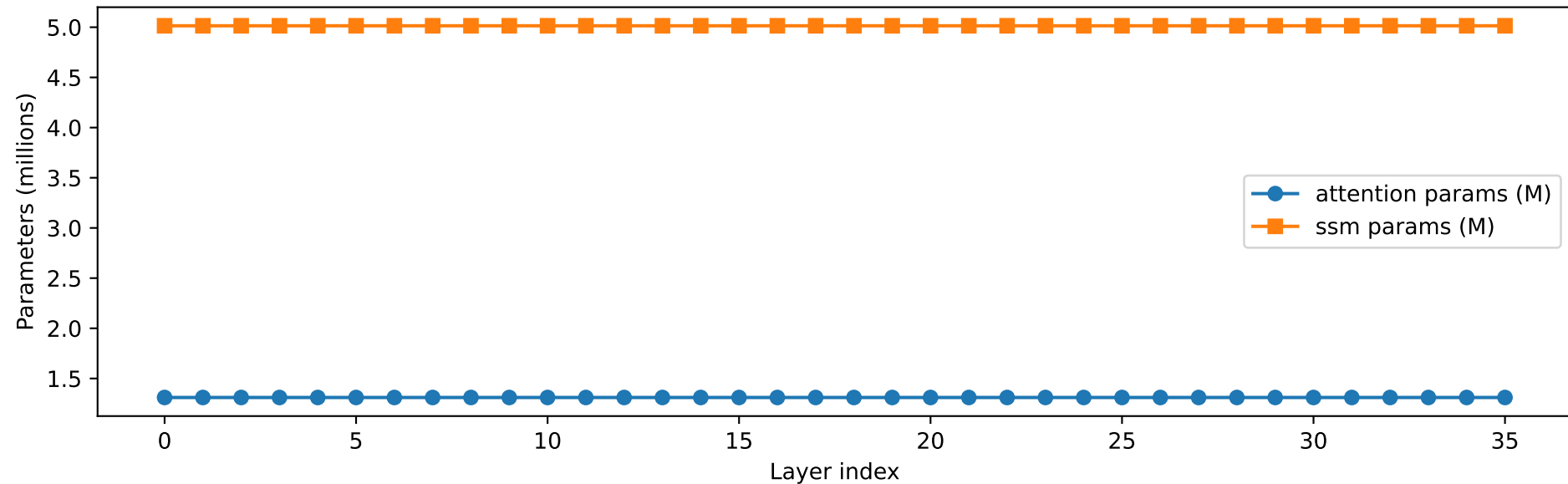
falcon-h1-0.5b: discovered component parameters by block
