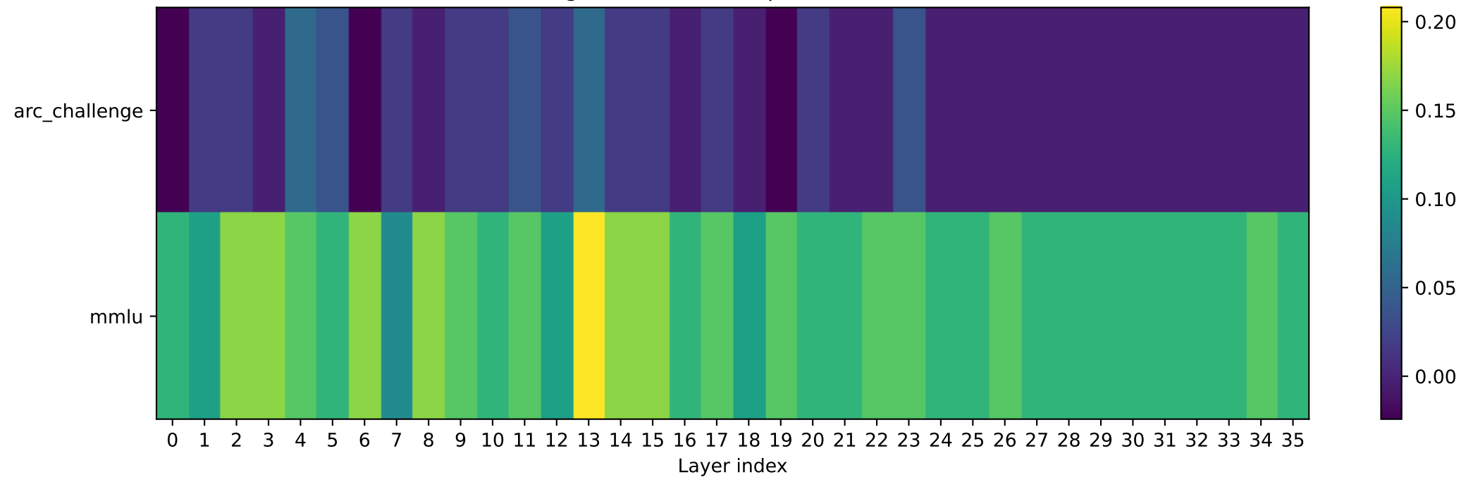
falcon-h1-0.5b: degradation heatmap for attention block ablations
