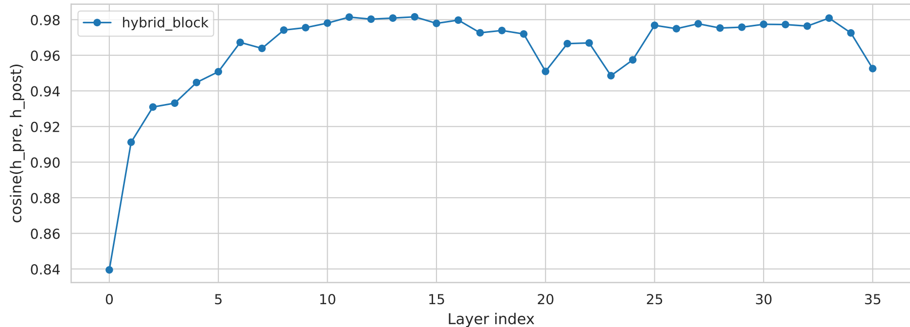
falcon-h1-0.5b: cosine similarity by layer
