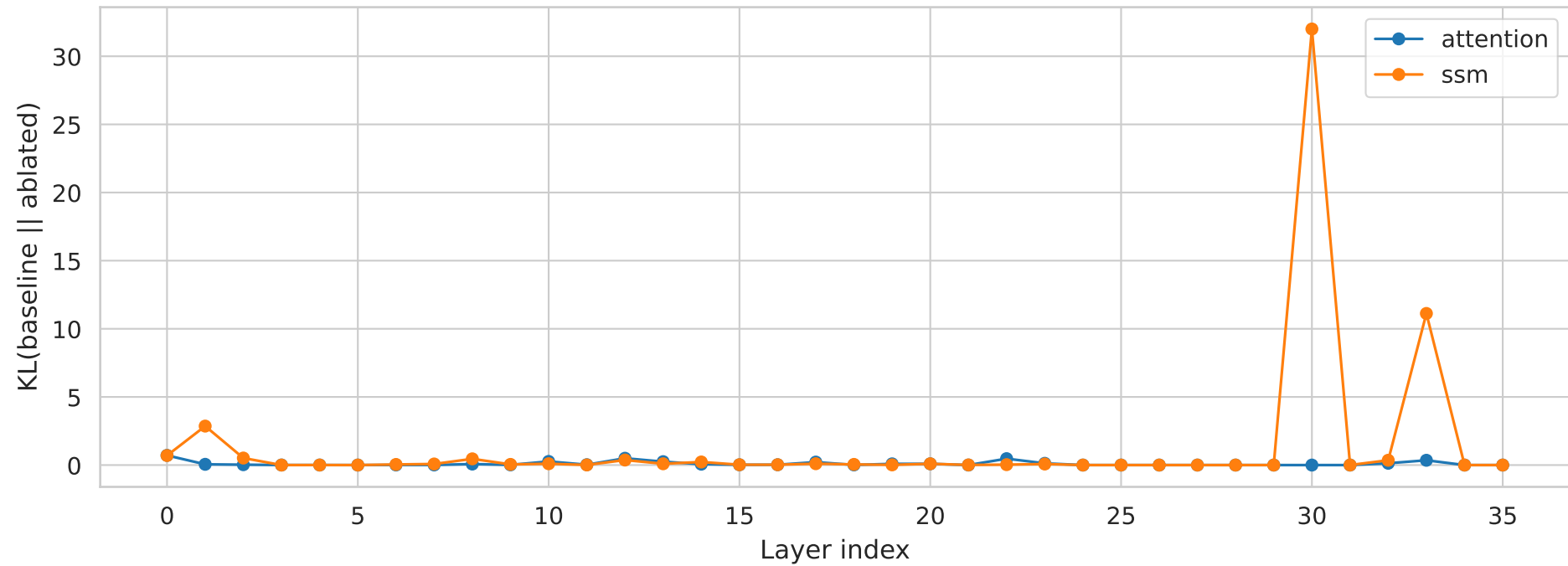
falcon-h1-0.5b: logit-lens divergence by layer
