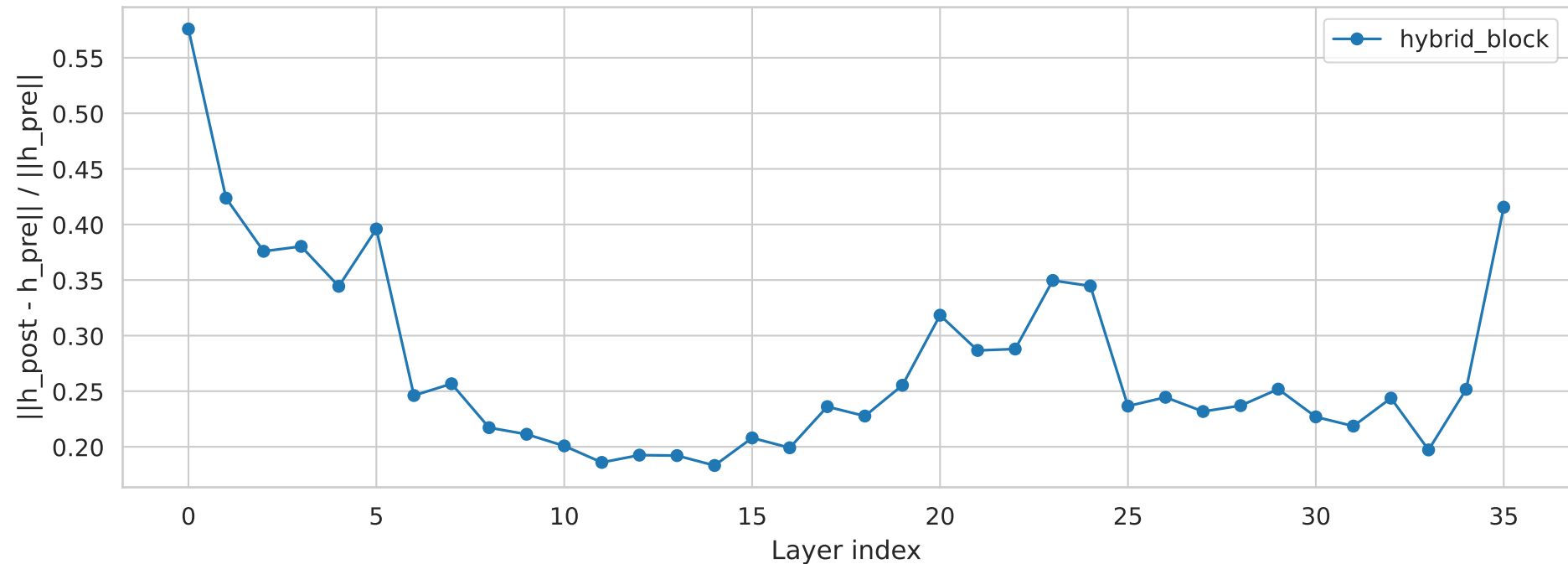
falcon-h1-0.5b: hidden-state norm change by layer
