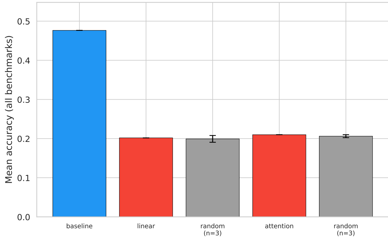
Qwen3.5-0.8B
