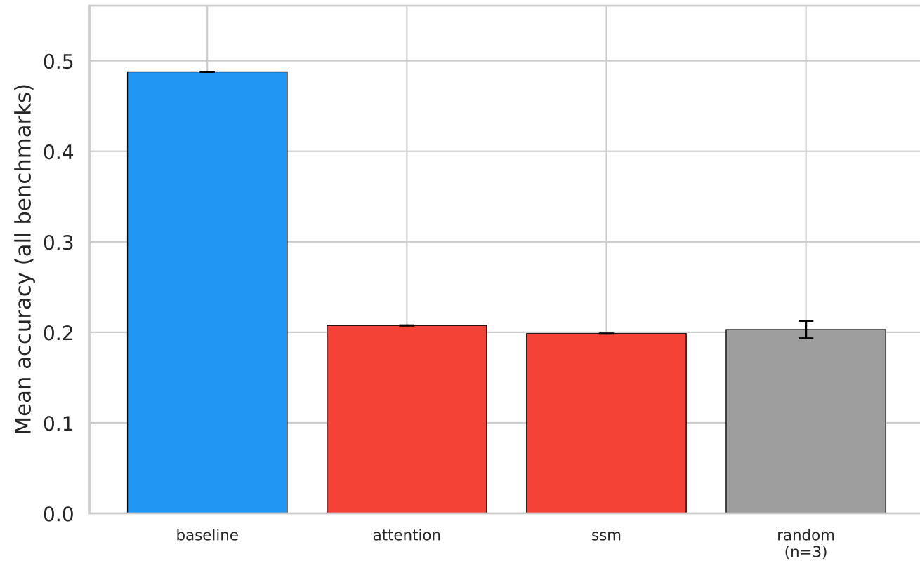
Falcon-H1-0.5B
