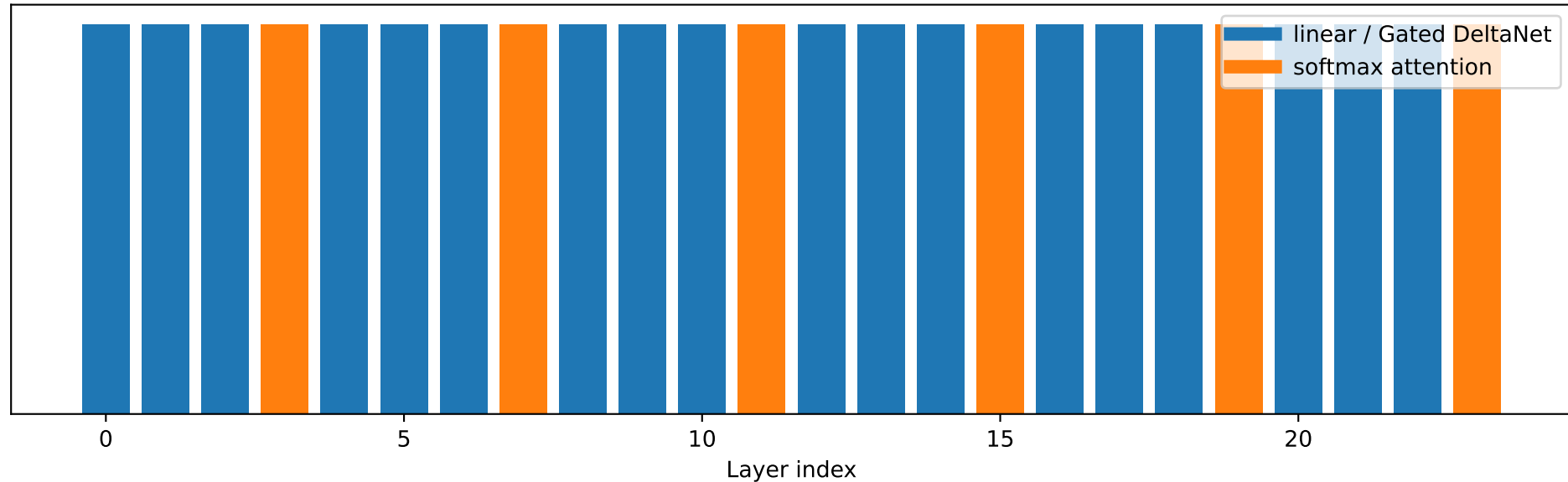
qwen3.5-0.8b: layer type distribution
