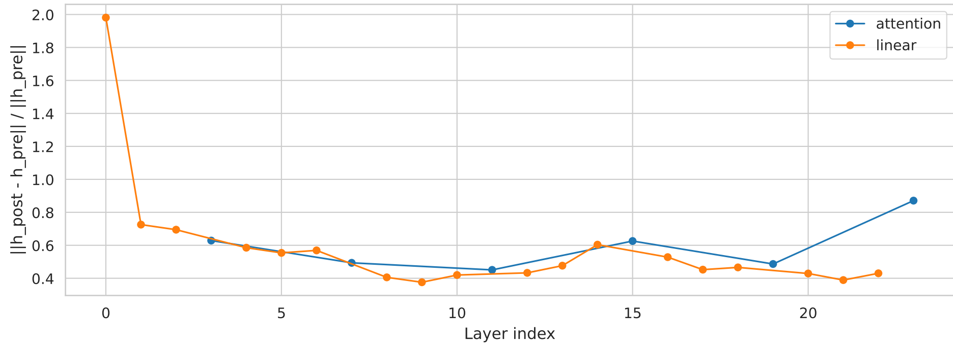
qwen3.5-0.8b: hidden-state norm change by layer
