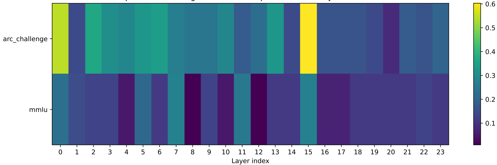
qwen3.5-0.8b: degradation heatmap for individual layer ablations
