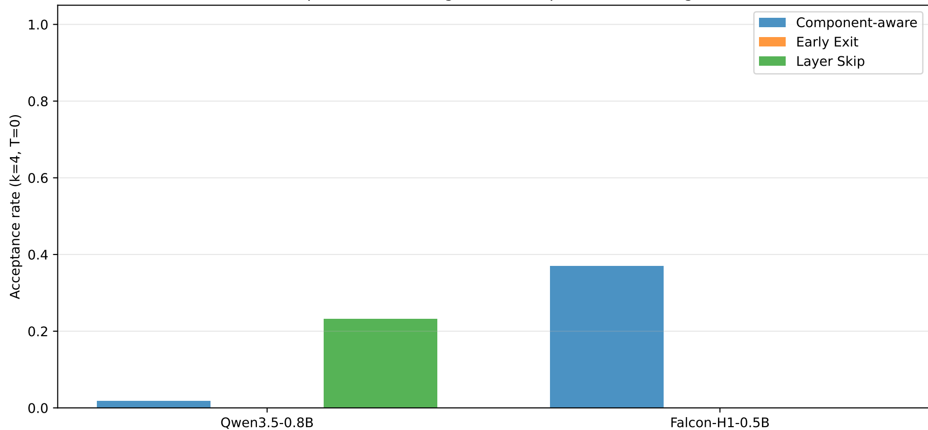
Component-aware vs generic self-speculation strategies
