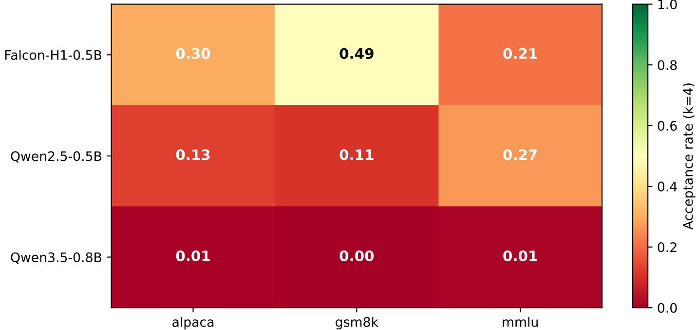
Task-dependent acceptance rate (greedy, k=4)
