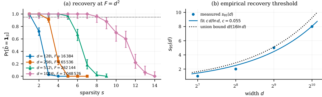
Figure 4: Threshold recovery at quadratic feature load, up to d = 1024 ( F = 1048576 ). (a) Empirical exact-recovery probability with Wilson 95% intervals; a fresh random code is drawn per trial. (b) The empirical threshold s_{95}(d) against the fitted c d / \ln d law and the conservative union-bound reference d / (16 \ln d) . Generated by scripts/make_figures.py from results/e6 .
