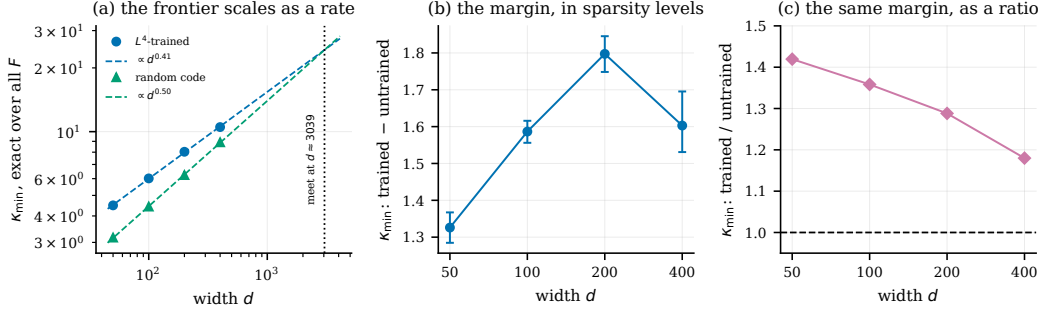
Figure 6: The frontier’s rate, and the margin it puts in question. All values are the exact \kappa_{\min} over every one of the F features, never the subset. (a) Both codes’ frontiers are close to straight on these axes over the four widths, and the untrained slope is the steeper. The power-law fits meet near d \approx 3039 , drawn to show what the two slopes imply and not offered as a prediction: it lies far outside the measured range, and four points do not identify the shape — other forms fit as well and move the meeting point by a factor of two. The robust statement is the ordering of the slopes, not where they cross. (b) The margin in sparsity levels, with two-sample bootstrap intervals over models; it peaks at d = 200 and the fall to d = 400 exceeds the sampling noise. (c) The same margin as a ratio, which falls at every step. The two panels are shown separately because they are the two honest readings of the same quantity and they do not agree until d = 400 .
