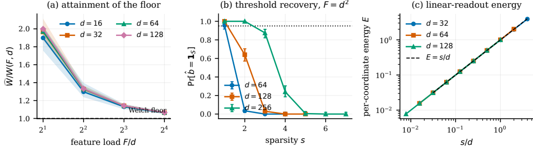
Figure 1: The Interface Diagnostic on random codes. (a) Attainment ratio \widehat{W}/W(F, d) of the calibrated tied readout versus feature load; shaded bands are the min-max range over trials, the dashed line is the floor of Theorem 5.1. (b) Exact threshold recovery at F = d^2 with Wilson 95% intervals; the dotted line marks the 0.95 level defining s_{95} . (c) Average per-coordinate linear energy under uniformly random supports against the s/d reference. Generated by scripts/make_figures.py from results/e1 , results/e2 and results/e3 .
