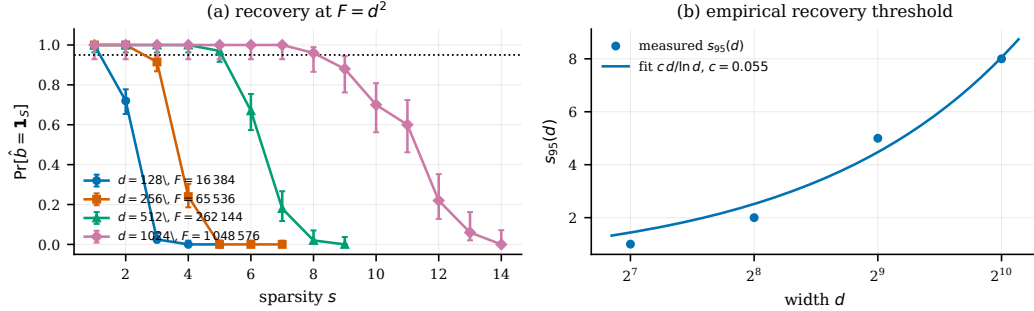
Figure 6: Threshold recovery at quadratic feature load, up to d = 1024 ( F = 1\,048\,576 ). (a) Empirical exact-recovery probability with Wilson 95% intervals; a fresh random code is drawn per trial. (b) The empirical threshold s_{95}(d) with the fitted c d / \ln d curve shown as a fit only: four widths do not distinguish it from c d or from c d / \ln^2 d , and no scaling law is claimed. Generated by scripts/make_figures.py from results/e6 .
