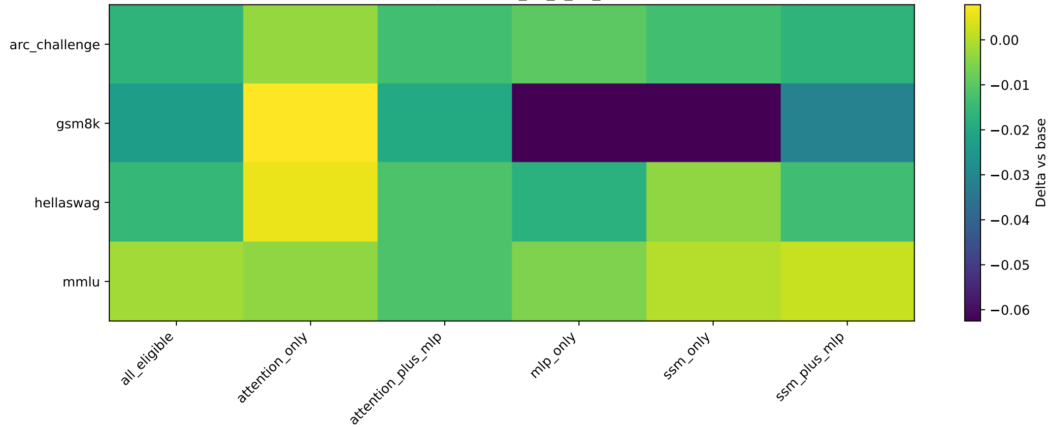
Benchmark x condition heatmap — falcon_h1_0_5b_base — trained on codealpaca
