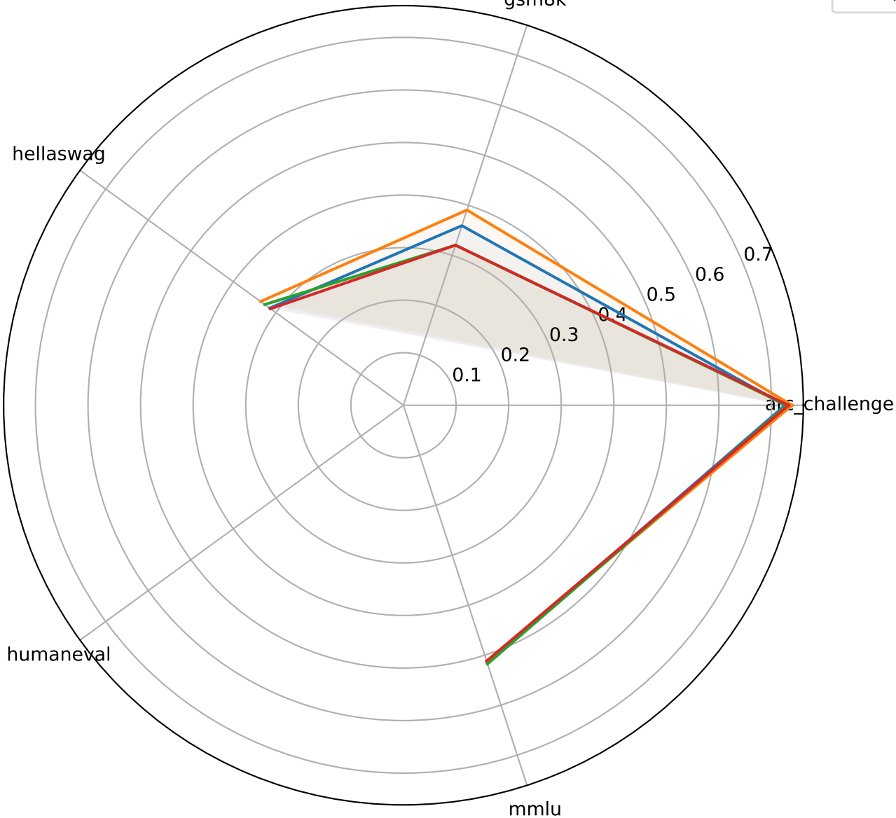
Benchmark radar — falcon_h1_0_5b_base — trained on codealpaca
