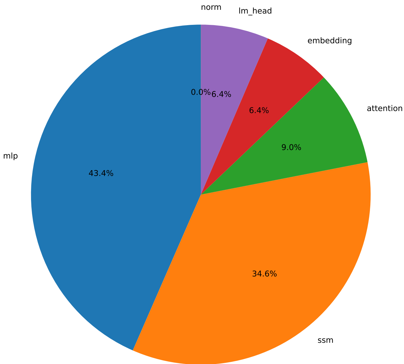
Parameter distribution by component — falcon_h1_0_5b_base
