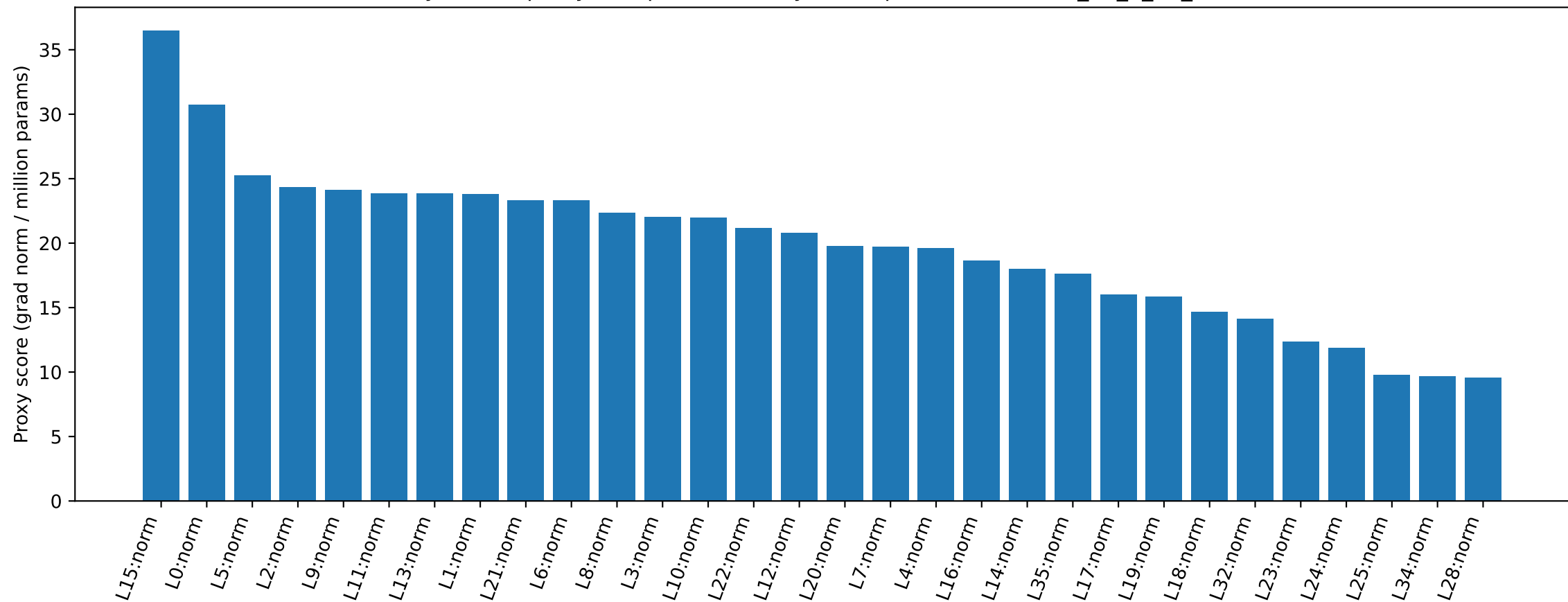
Layer Card proxy — top sensitive layer/components — falcon_h1_0_5b_base
