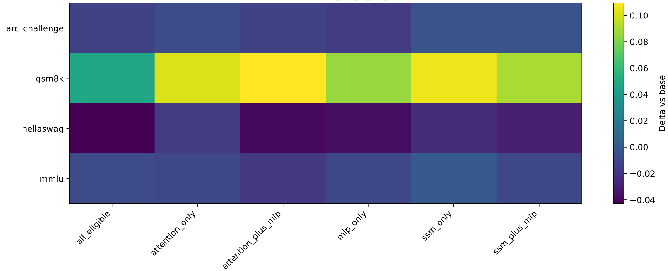
Benchmark x condition heatmap — falcon_h1_0_5b_base — trained on ultrachat
