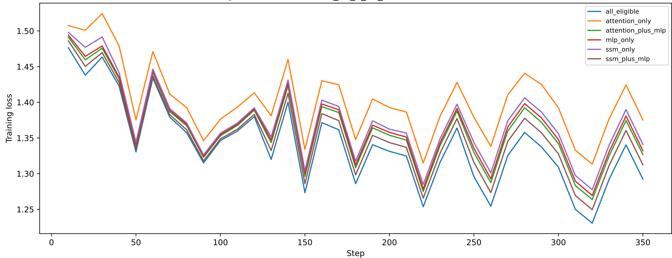
Training loss curves — falcon_h1_0_5b_base — trained on ultrachat
