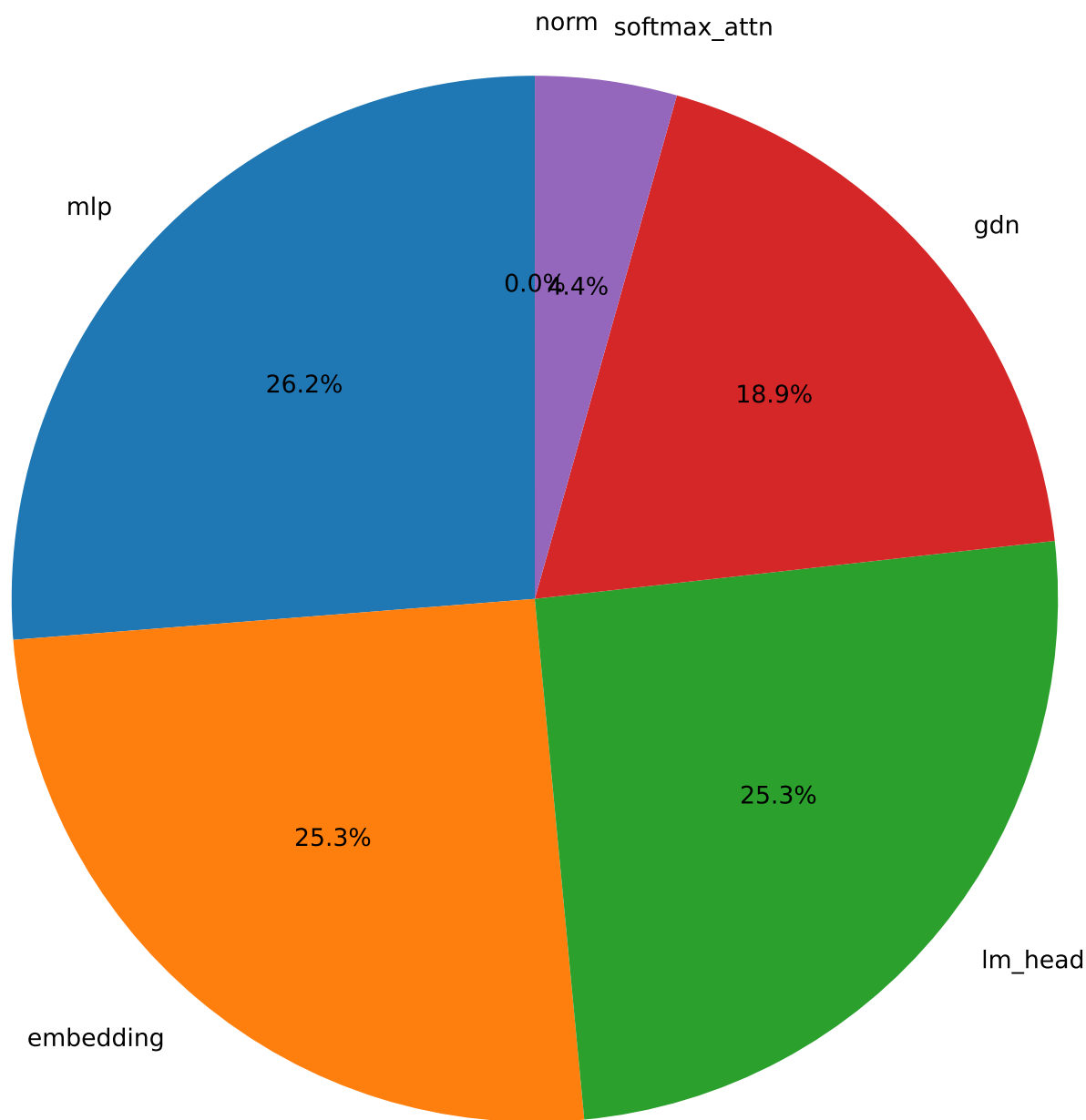
Parameter distribution by component — qwen3_5_0_8b_base
