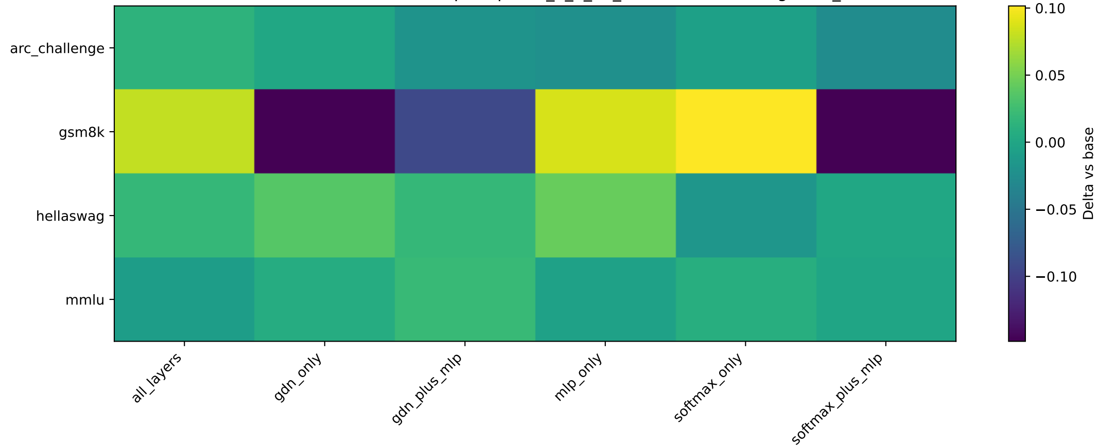
Benchmark x condition heatmap — qwen3_5_0_8b_base — trained on gsm8k_train
