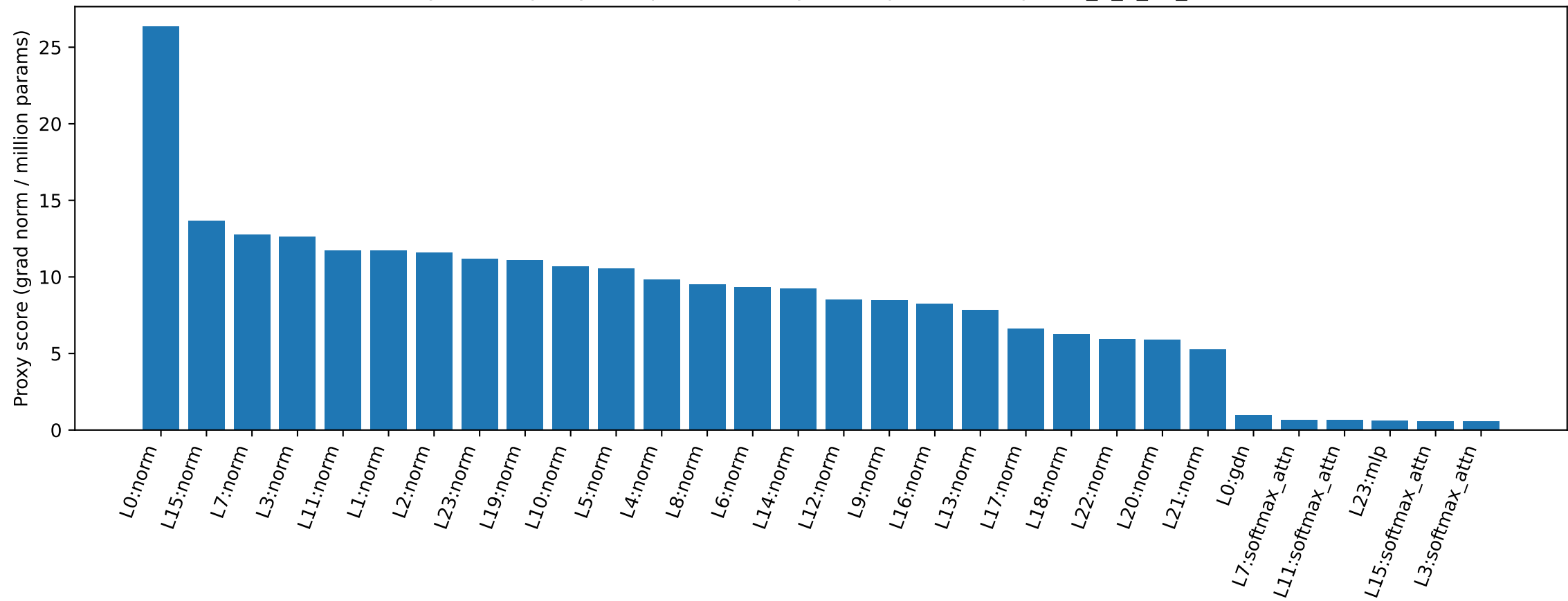
Layer Card proxy — top sensitive layer/components — qwen3_5_0_8b_base
