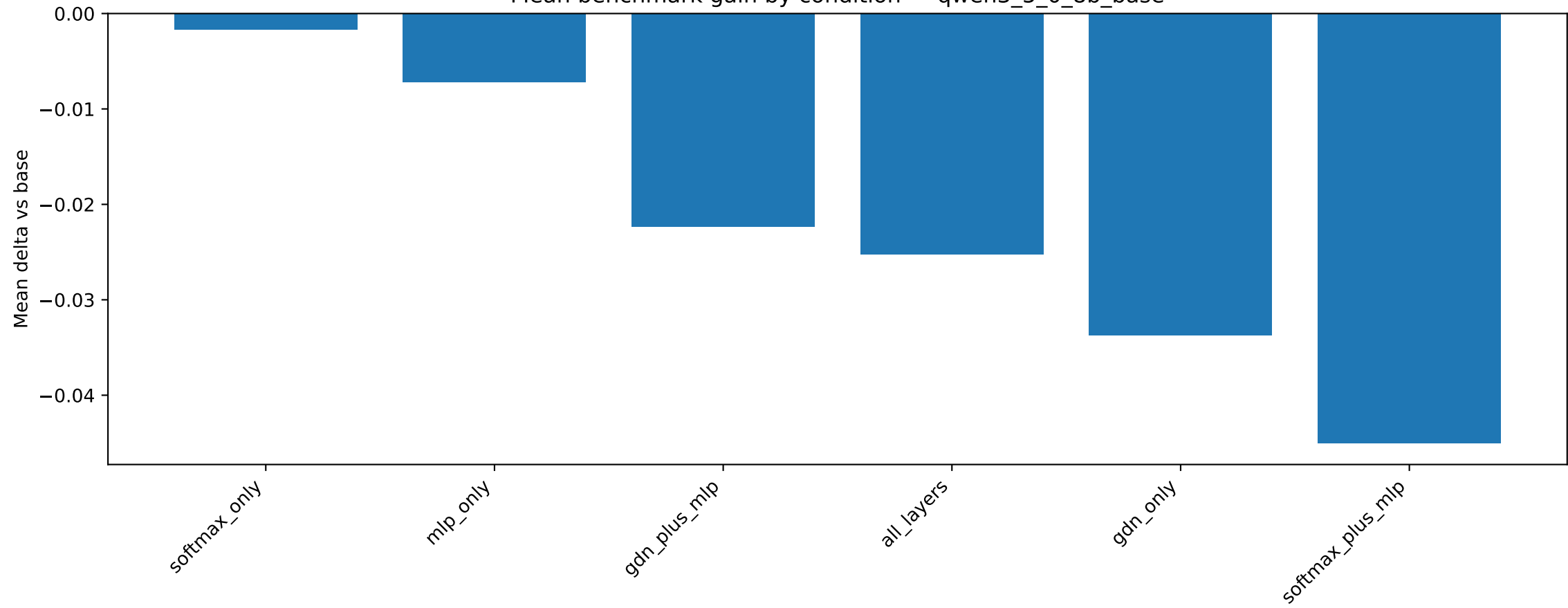
Mean benchmark gain by condition — qwen3_5_0_8b_base
