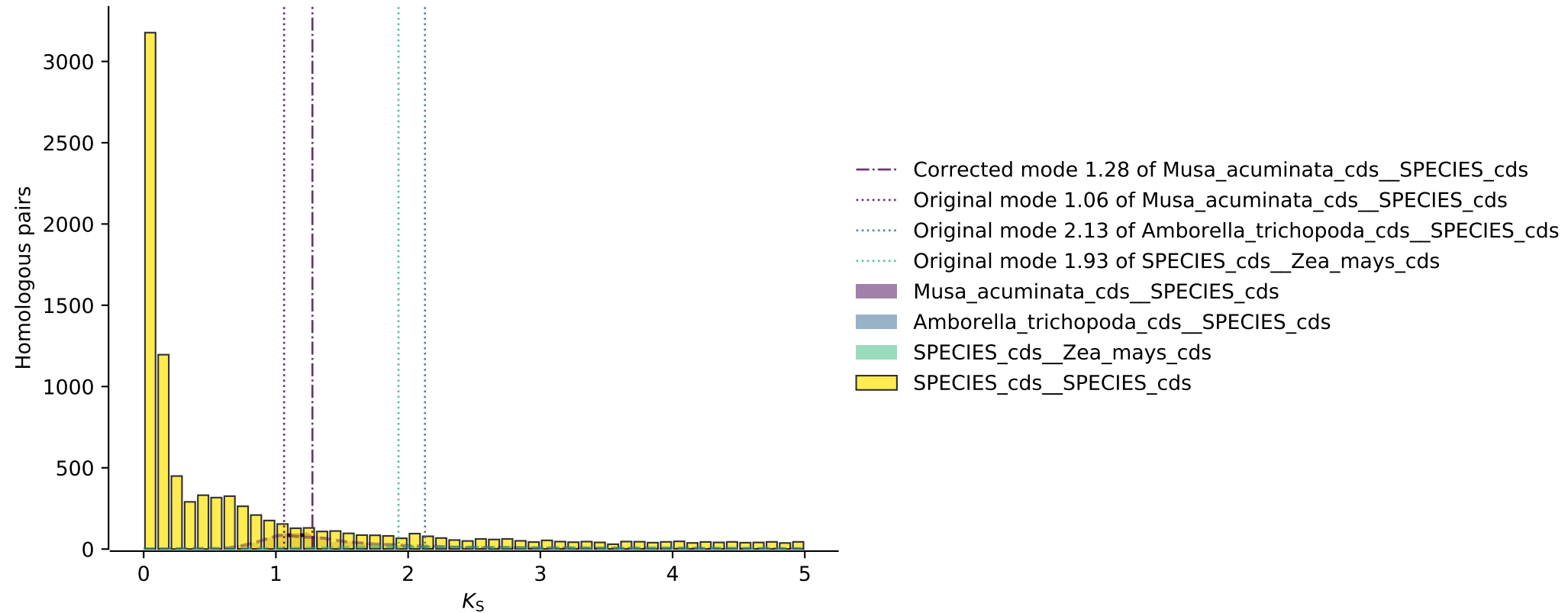
Corrected K_S distribution of SPECIES_cds
