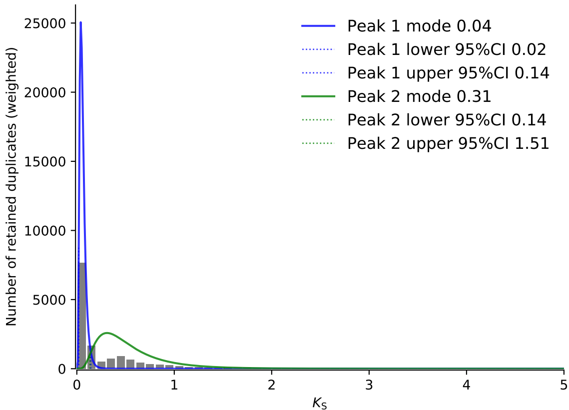
Anchor K_S distribution of final_true_cds_WH_single.fasta.tsv.ks.tsv
