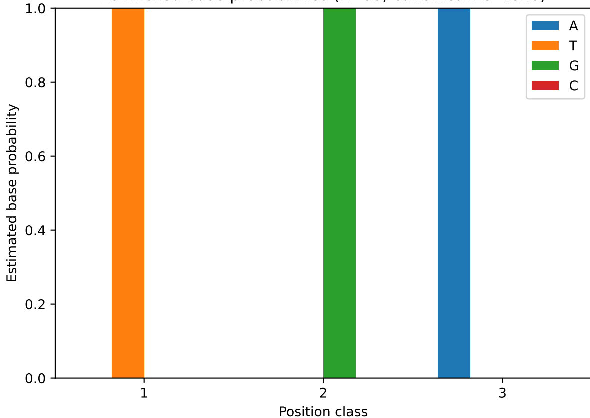
Estimated base probabilities (L=60; canonicalize=full6)
