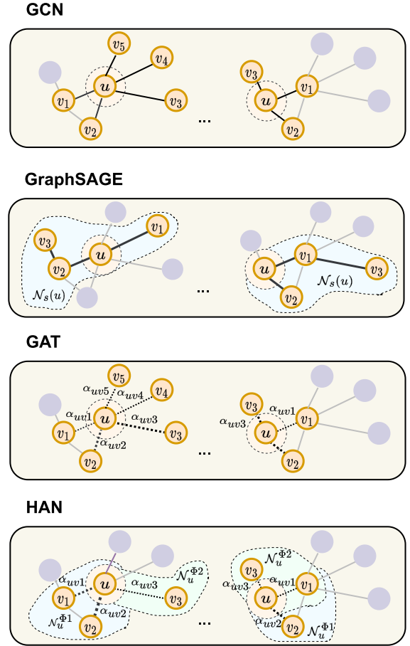
FIGURE 2. Illustration of common GNNs used in literature. GCN aggregates its 1-hop neighborhood; GraphSAGE samples a fixed number of neighbors and aggregates them; GAT leverages the attention mechanism to weight neighbors depending on their importance; HAN applies attention to heterogeneous graphs by learning attention weights between nodes from a same meta-path.
