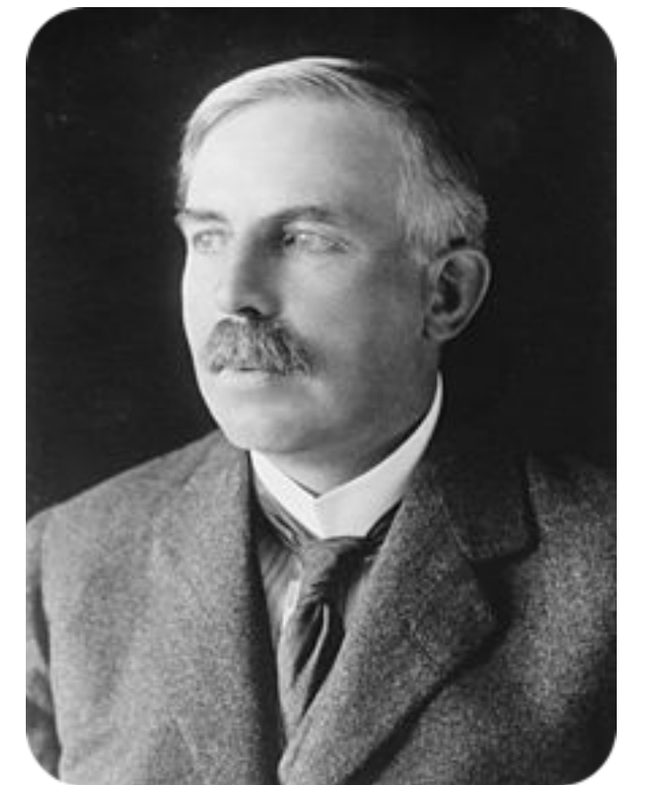
Ernest Rutherford 1871 - 1937
