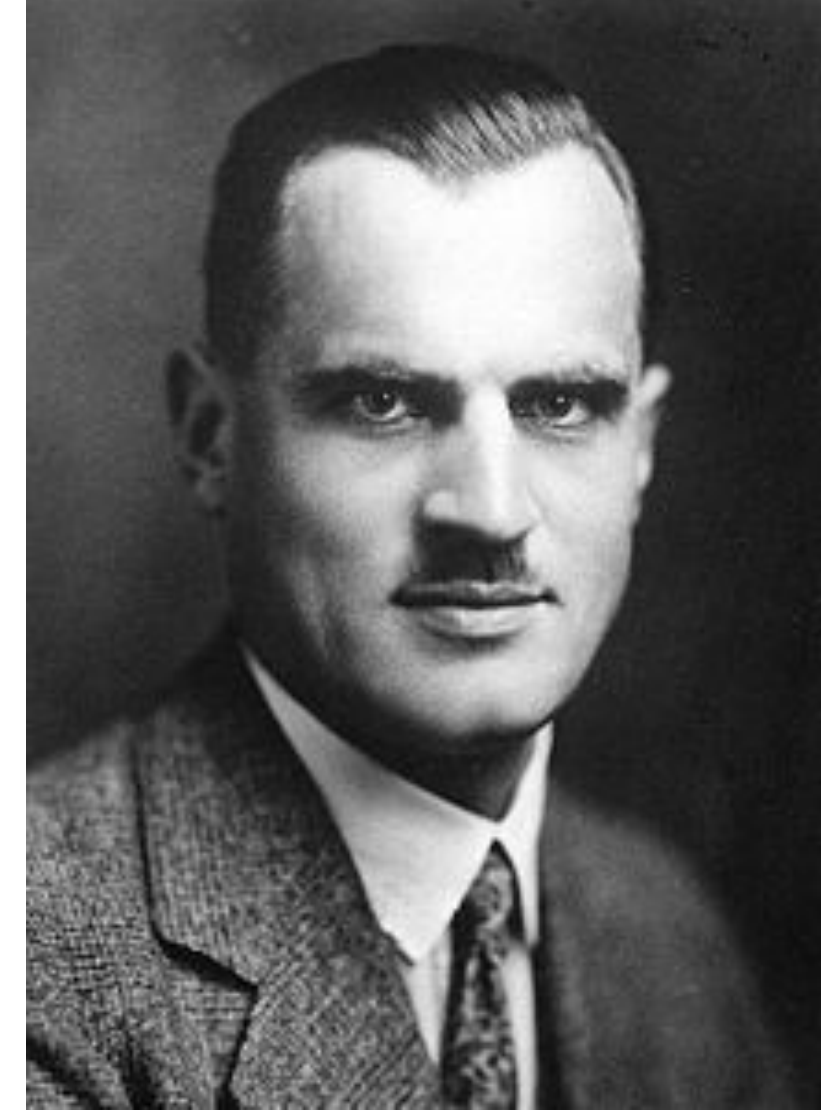
Arthur Compton 1892 - 1962
