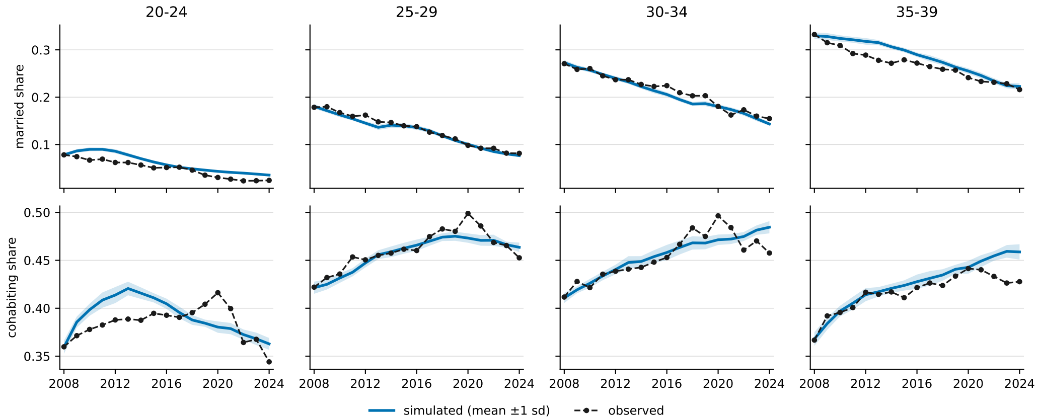
COL — union composition by age band, women 20-39: no-reflexivity model vs observed
