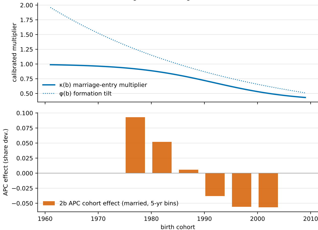
CRI — calibrated cohort gradient vs Stage 2b APC cohort effects (married)
