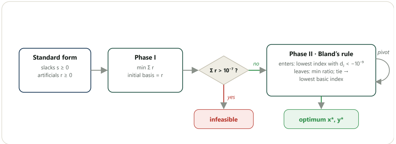
FIGURE 3 Two-phase simplex flow. Tolerances are those in the RatioAvis 1.1.1 source code.
